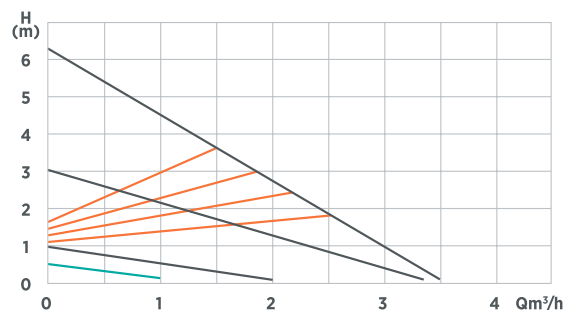
Characteristic WITA Delta HE 55
