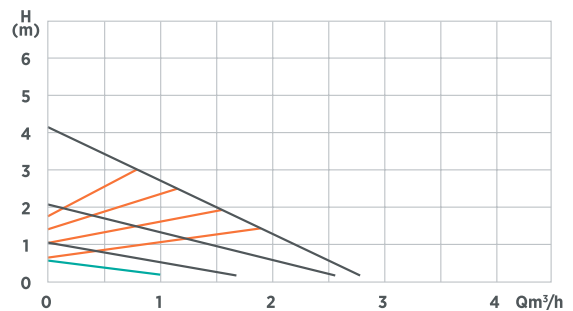
Characteristic WITA Delta HE 35
